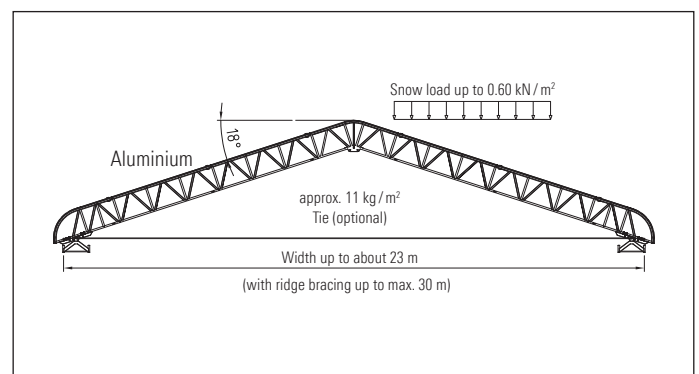
Keder Roof XL for wintertime timber construction work
