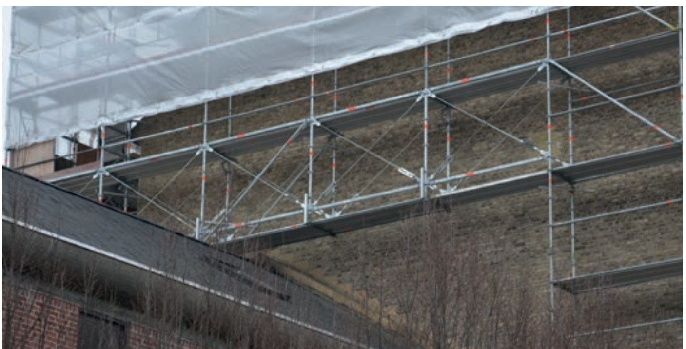
Bridging / supporting of work scaffolding using an external and non-loadable roof
