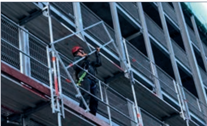
SpeedyScaf assembly with I-Guardrail
