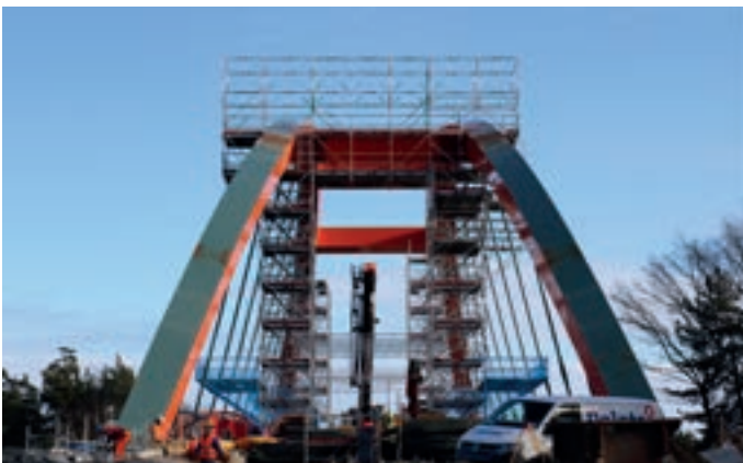
Self-supporting work scaffolding between the arches of an arched bridge with Allround FW System
