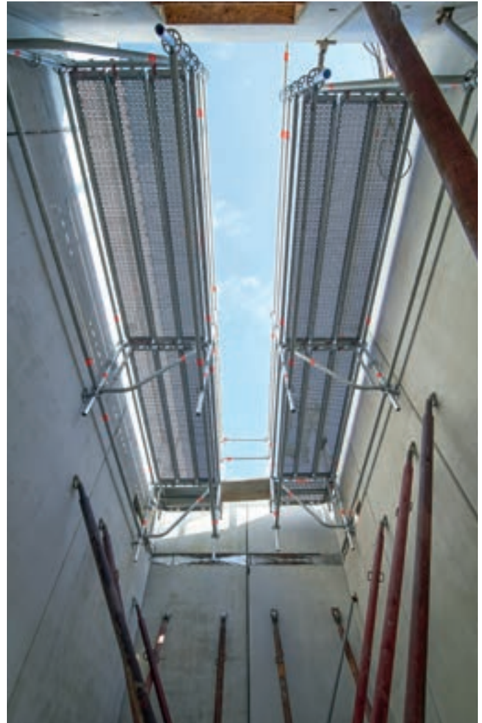
The space underneath the scaffolding remains free for the push-pull props
